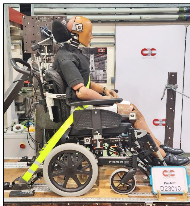
D23-010 Baseline Test, Surrogate Vehicle Anchored Occupant Restraint System Layout
